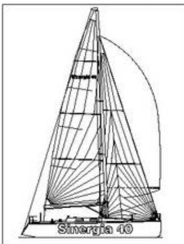
sailplan
