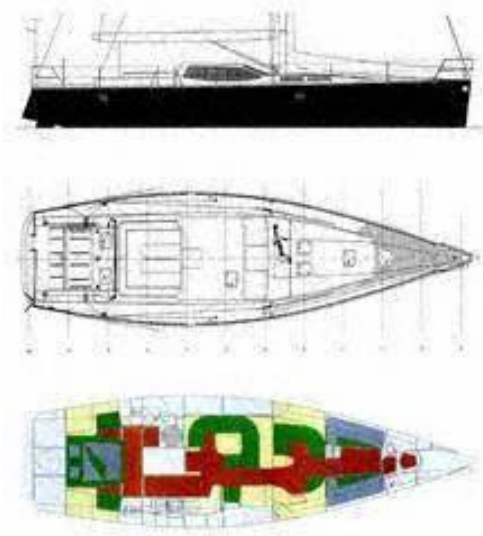
Interior & deck layout
